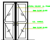
FRONT ELEVATION
