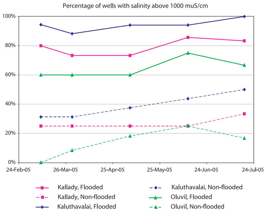
Figure 32. Percentage of wells with salinity above the drinking water thresholds a function of time after the tsunami
