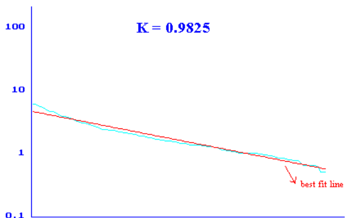
Figure 2.8: AWBM Catchment Water Balance Programme graphical determination of baseflow recession constant, K
