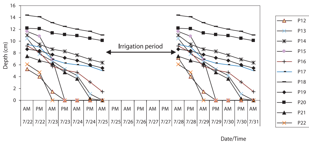
FIGURE 13. Evolution of water depth in the fields (peg nos. 12 to 22).
