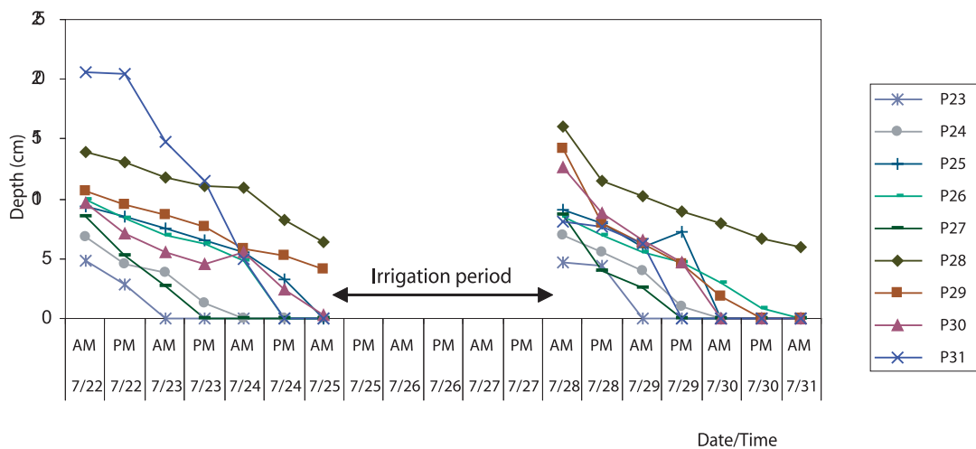
FIGURE 14. Evolution of water depth in the fields (peg nos. 23 to 31).
