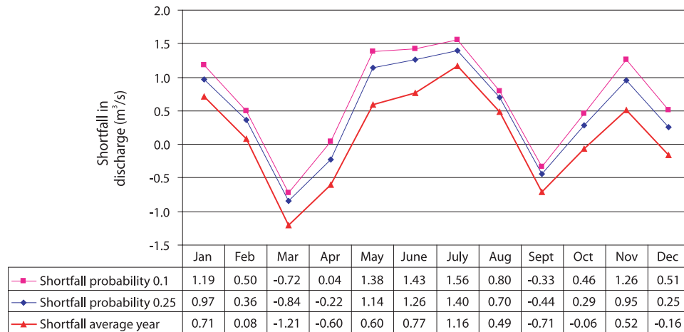
FIGURE 6. Shortfall in irrigation needs to be met by dam releases.
