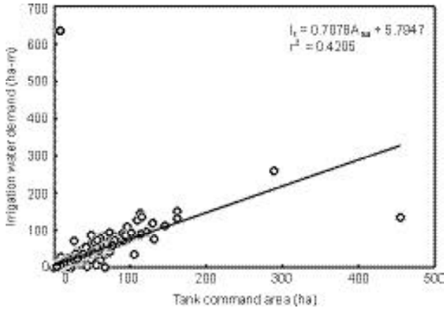
FIGURE 3. Irrigation water demand ( I_t ) versus tank command area ( A_{tco} ).
