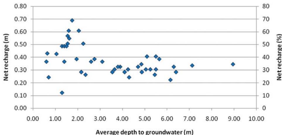
FIGURE 2.8. Relationship between average depth to groundwater and net recharge during wet months.
