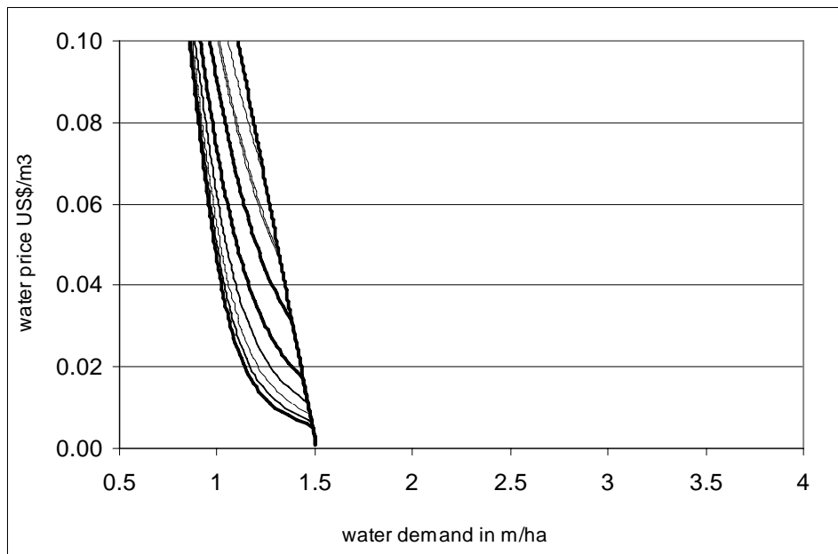
Figure 6: Demand curves for efficiency range 60% - 80%
