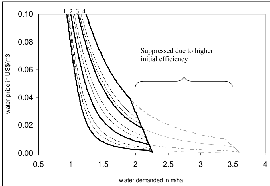
Figure 6: Demand curves for efficiency range 60% - 80%
