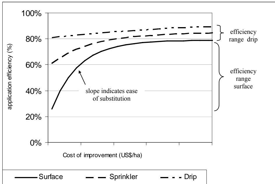
Figure 1: Application efficiency cost curves
