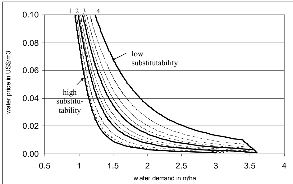
Figure 4: Demand curves for efficiency range 25%-80%
