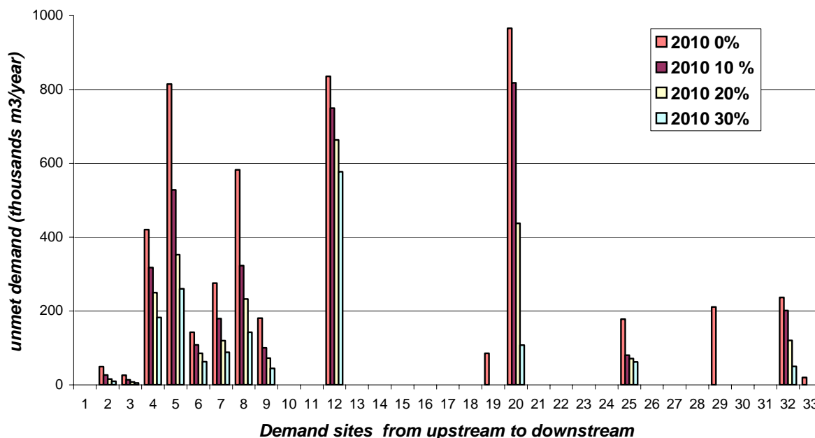
Figure 6: Annual unmet demand (in thousands m 3 ) from WEAP simulations over 15 normal years with Water Demand Management (WDM)
