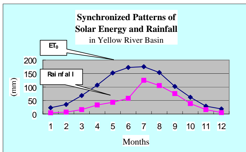
Figure 2. Solar Energy and Rainfall in Yellow River Basin
