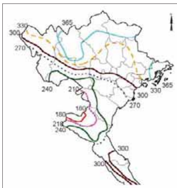
Figure 2. Length of growing season in Vietnam.
