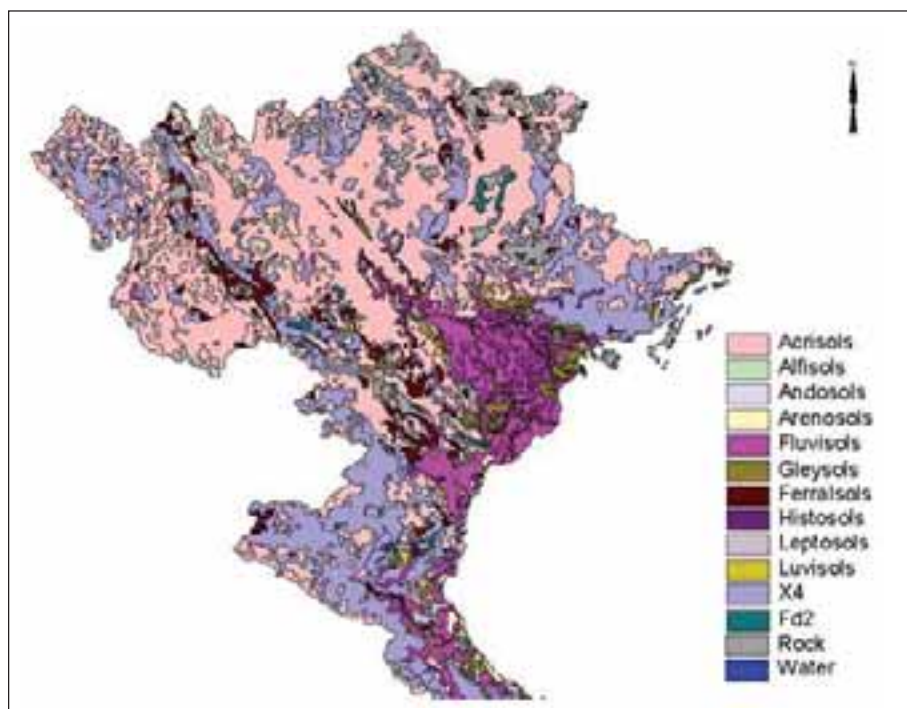
Figure 3. Soils of northern Vietnam.
