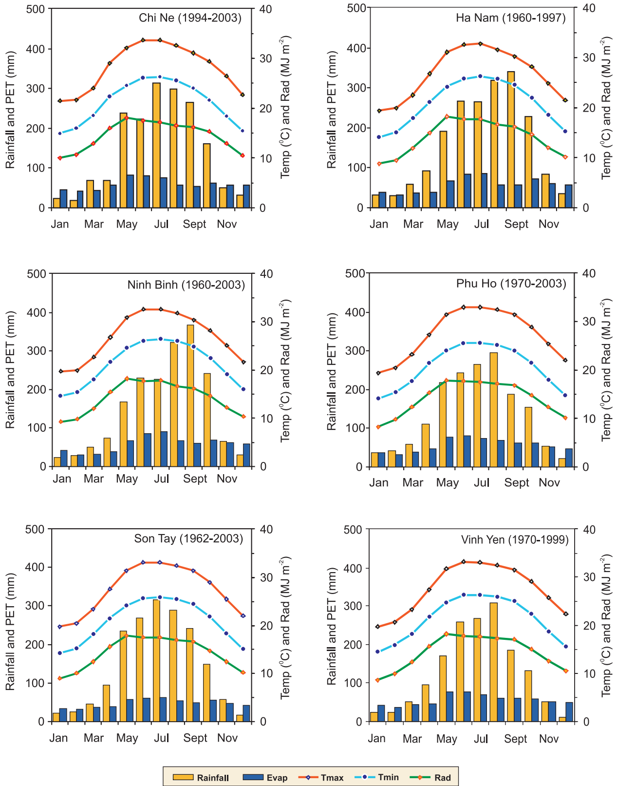
Figure 8. Monthly average rainfall (mm), potential evapo-transpiration (mm), maximum and minimum temperatures (°C) and solar radiation (MJ m -2 ) of sites located in the six provinces of northern Vietnam.
