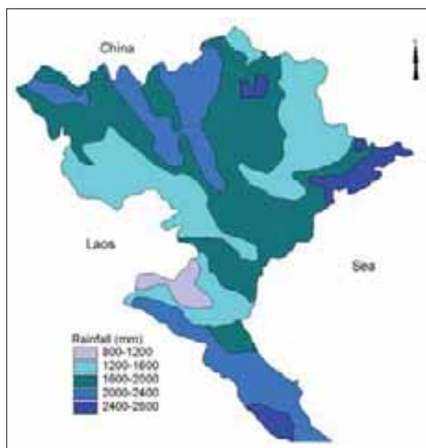
Figure 1. Annual rainfall in northern Vietnam.
