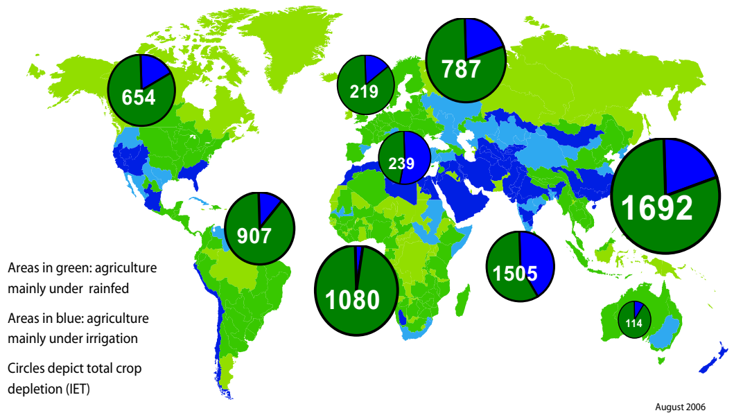
Map 1. Green water accounts for 80% of crop use, irrigated water 20%, with big regional variations.
