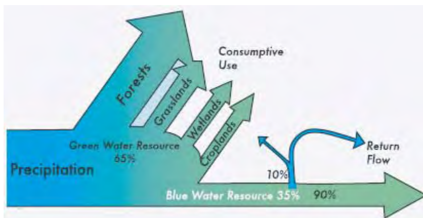
Figure 4. Global water balance
