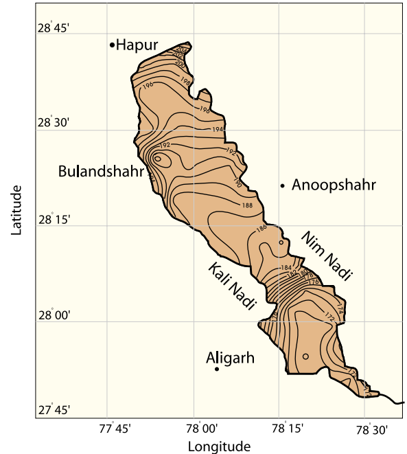
Figure 1. Water table elevation contours (meters above sea level) Post Monsoon 1984.
